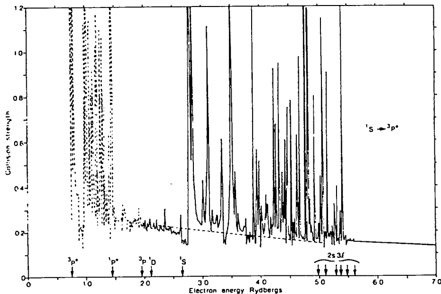
Fig. 3. Resonance structure in the 0 V ( 2s^2 1S - 2s 2p^3 P^0 ) collision strength, from the calculations of Berrington et. al.
